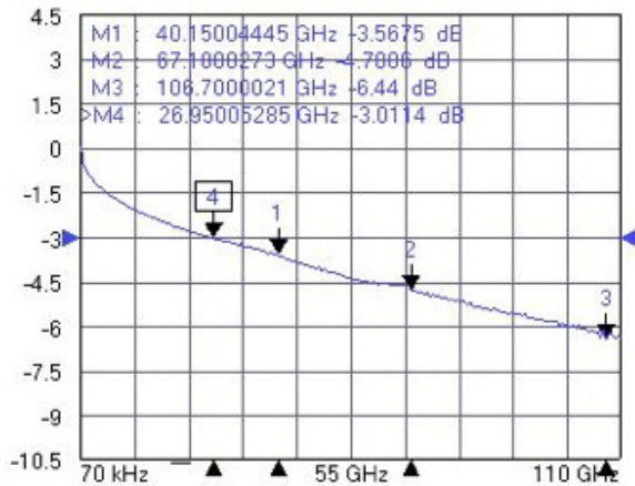
Tr3 S21 Trans LogM RefLvl: -3 dB Res: 1.5 dB/Div
