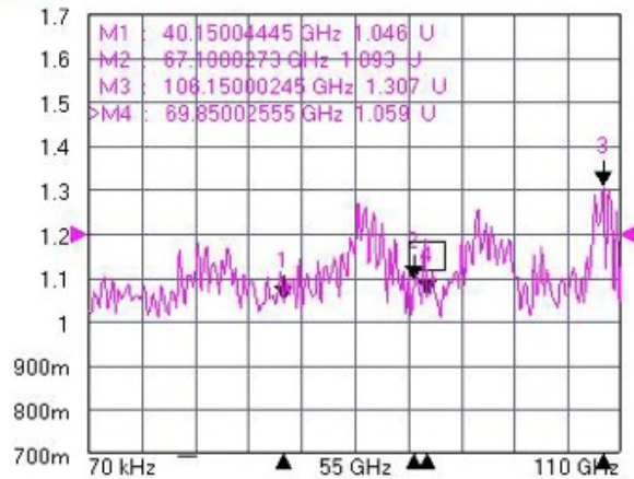
Tr4 S22 Refl SWR RefLvl: 1.2 U Res: 100 mU/Div
